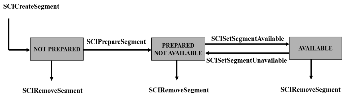
Figure 1 - State machine for a local segment
