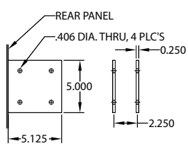
Medium Voltage Output Bus: Models 80 Vdc to 1000 Vdc
