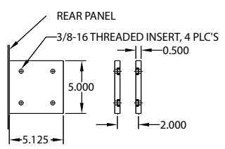
Low Voltage Output Bus: Models 50 Vdc and below
