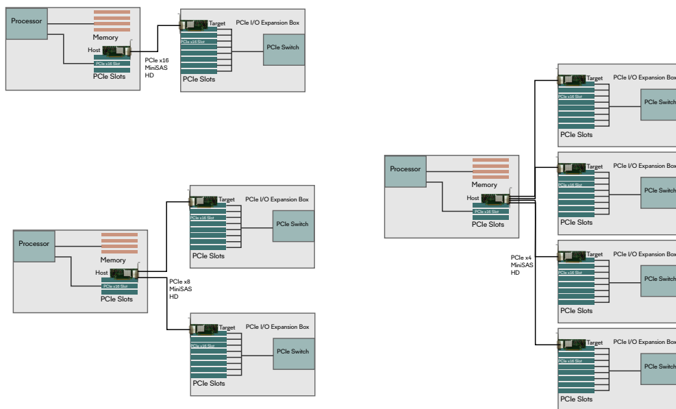
Figure 1:PXH832 I/O Expansion Configurations
