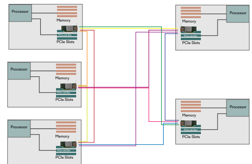
Five node MXH930 cluster
